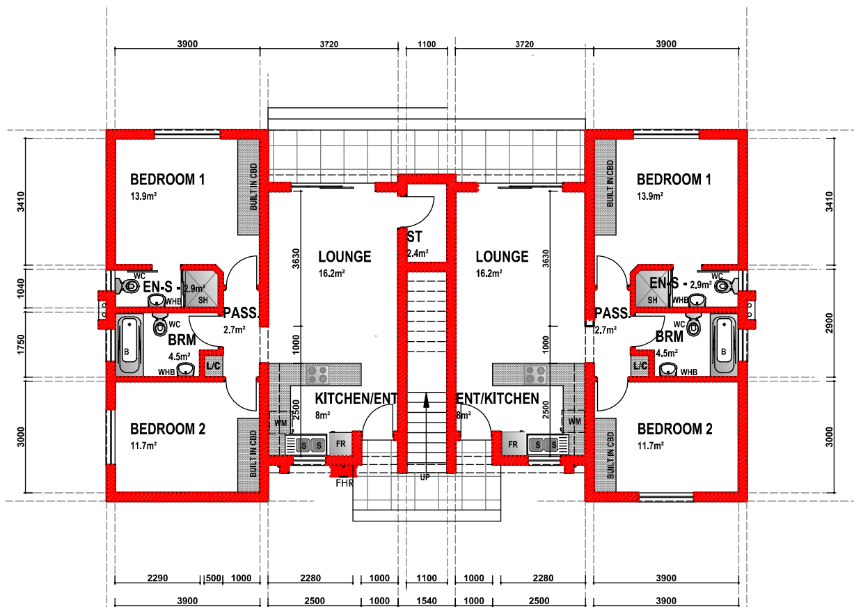
GROUND FLOOR PLAN - TYPE B SCALE 1:100
