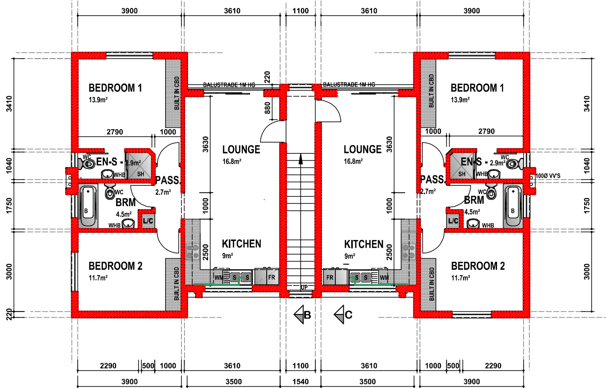
FIRST FLOOR PLAN - TYPE B SCALE 1:100
