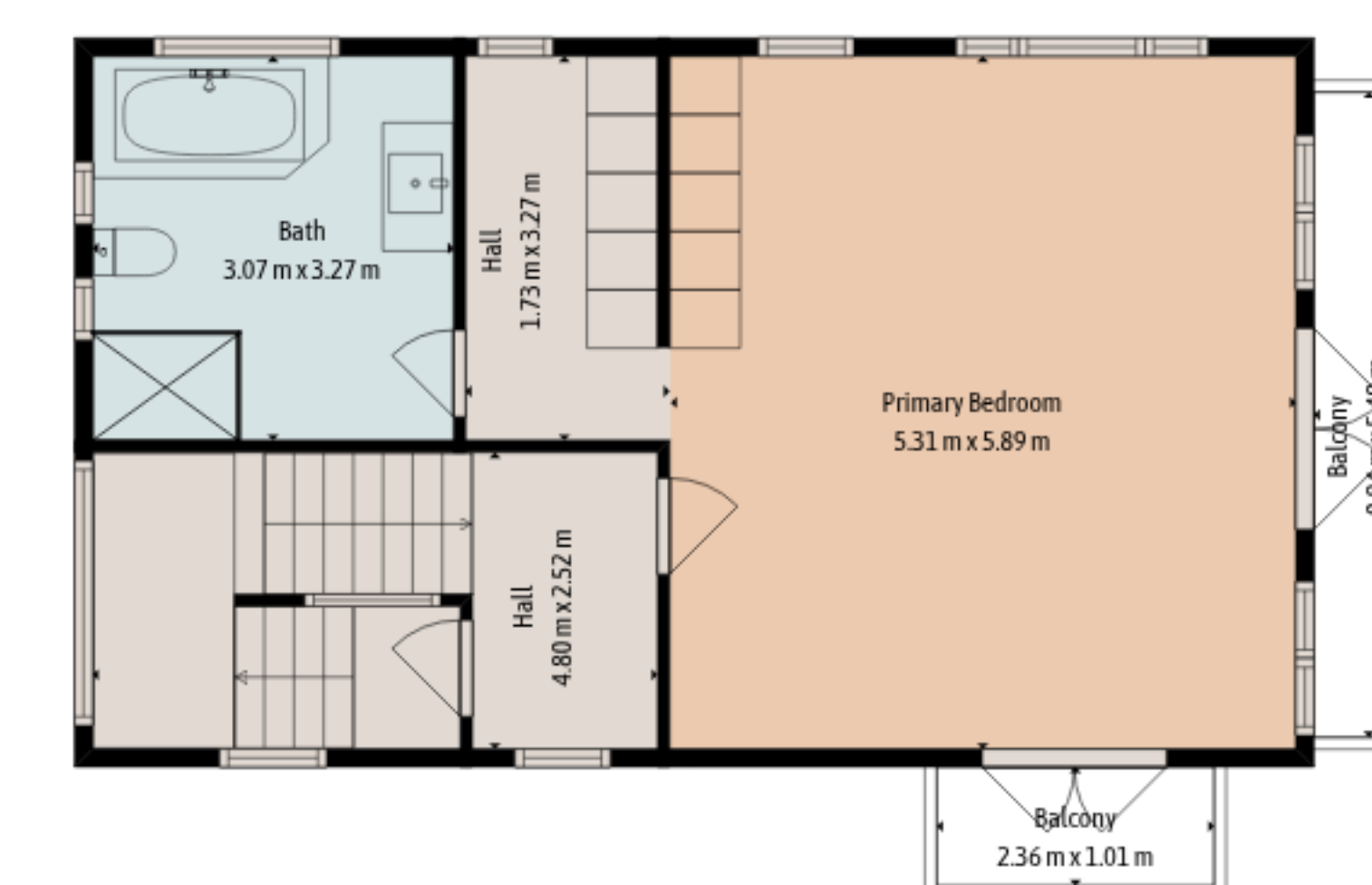
3rd Floor
