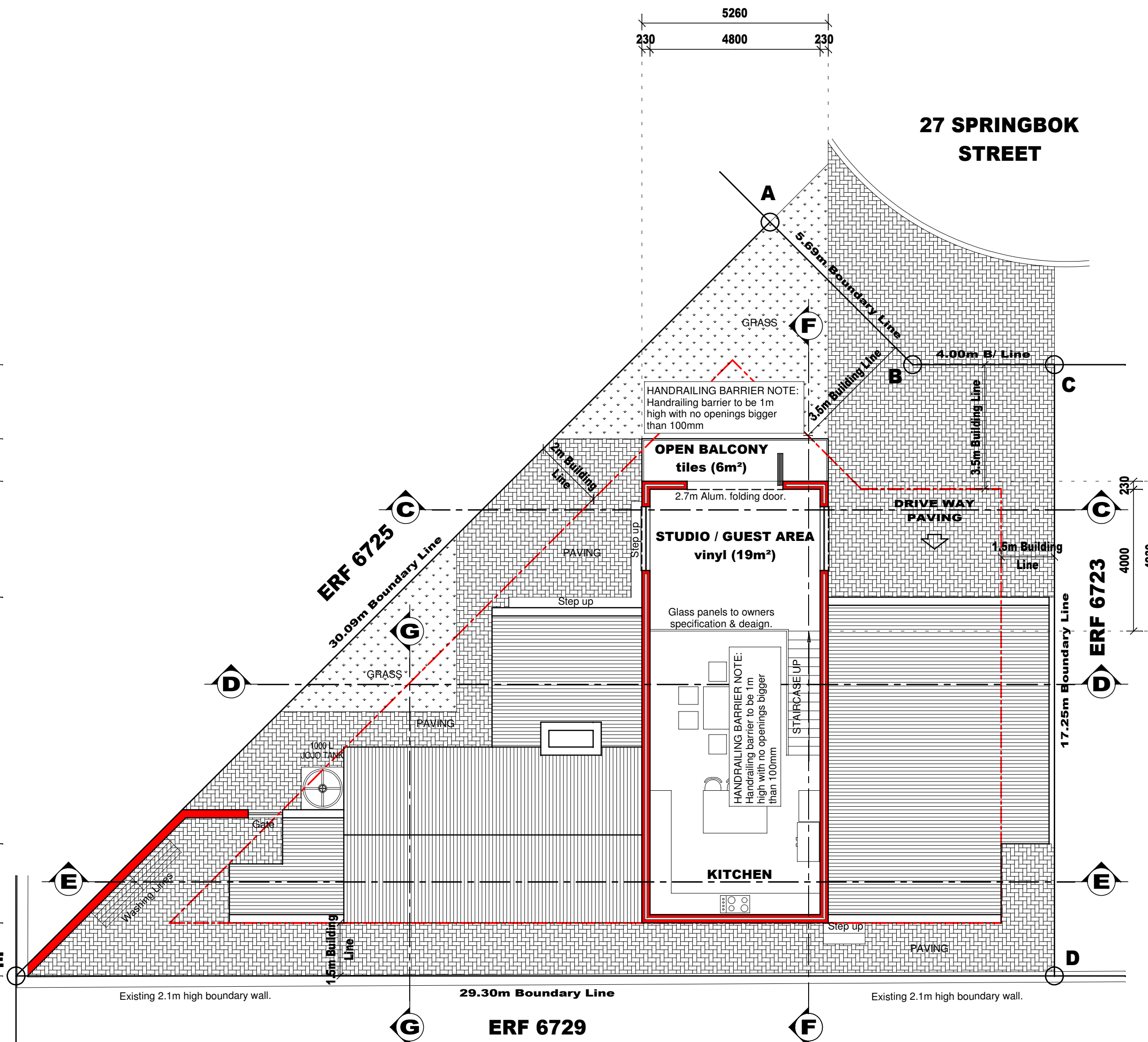
LOFT AREA LAYOUT PLAN scale 1:100
