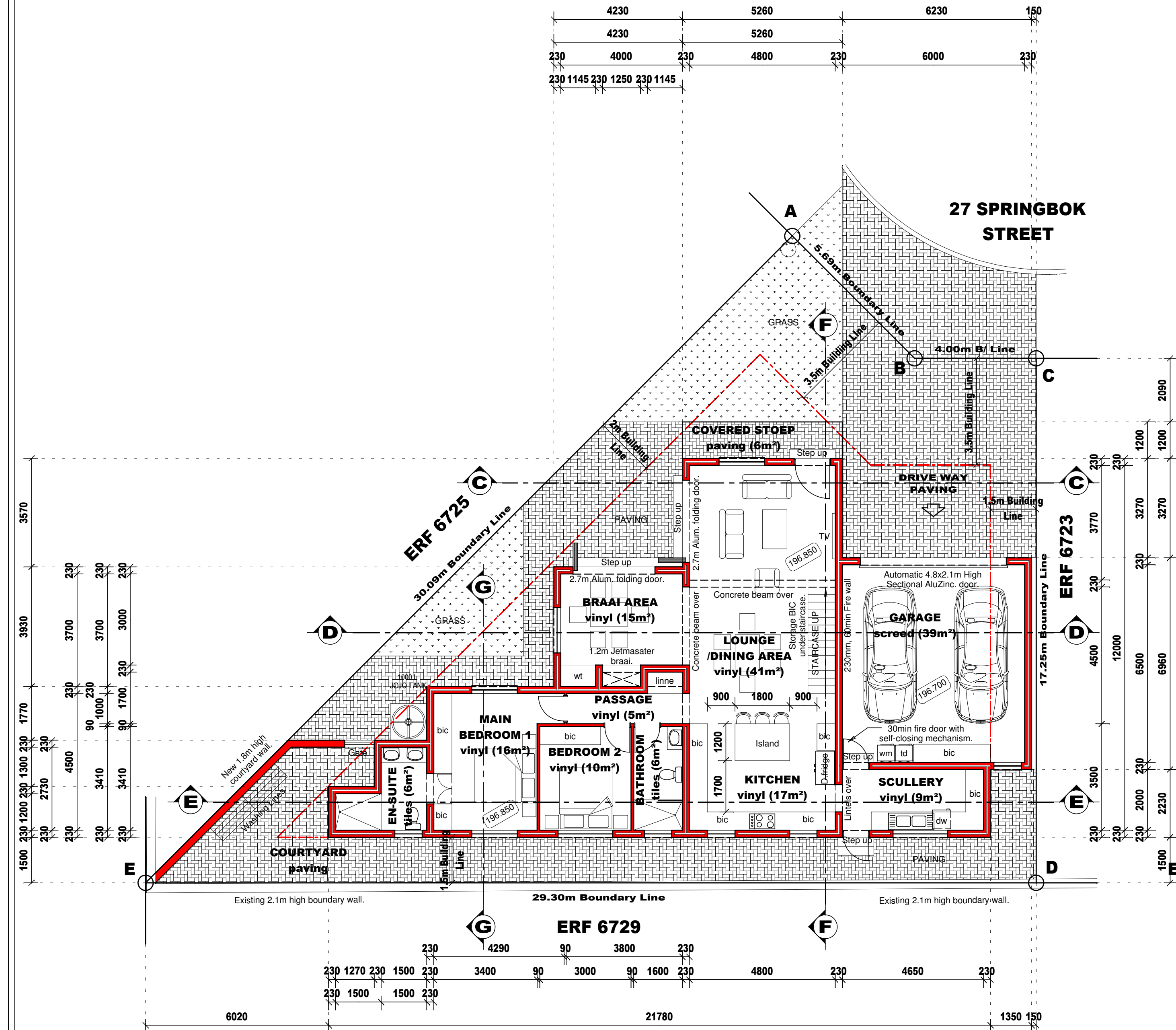
GROUND STOREY LAYOUT PLAN scale 1:100
