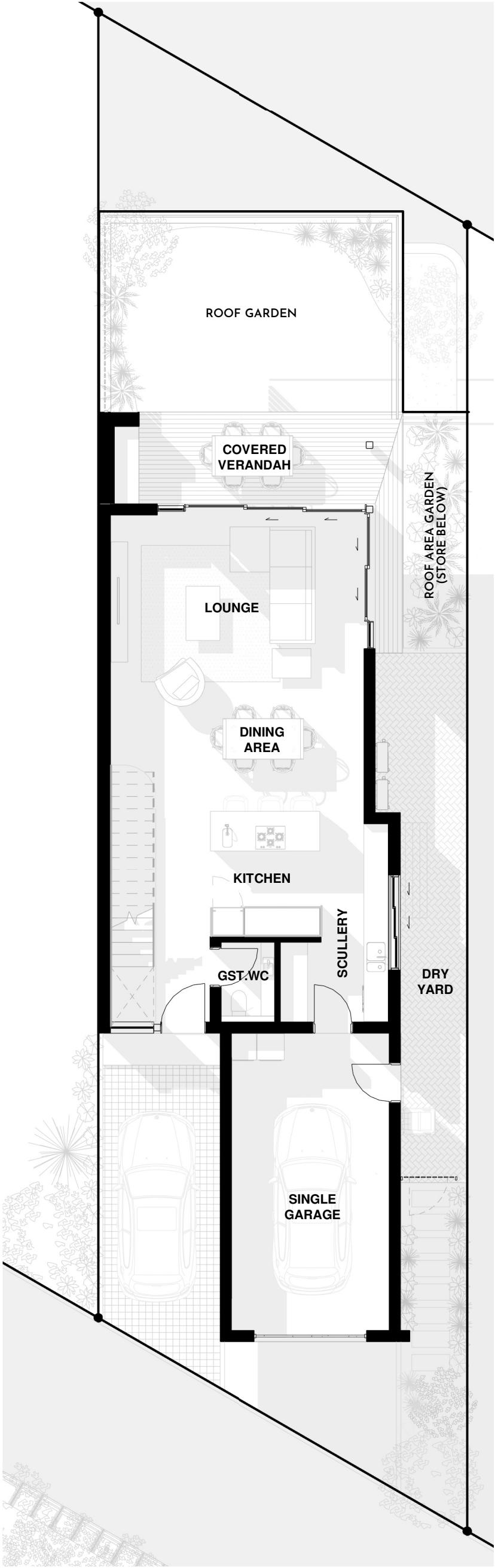
GROUND FLOOR - DUPLEX TYPE D
