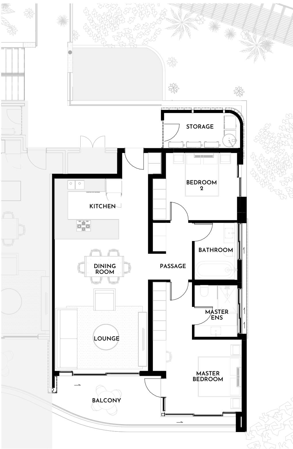
FIRST & SECOND FLOOR UNITS-UNIT TYPE B- LEFT SCALE 1 : 100
