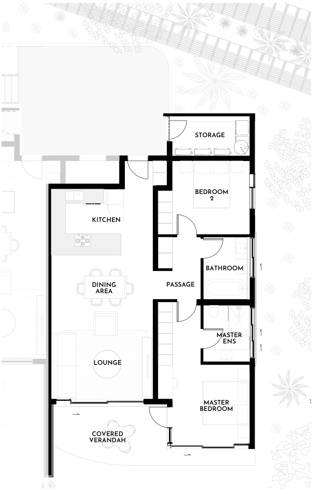
GROUND FLOOR -UNIT TYPE B- LEFT SCALE 1 : 100
