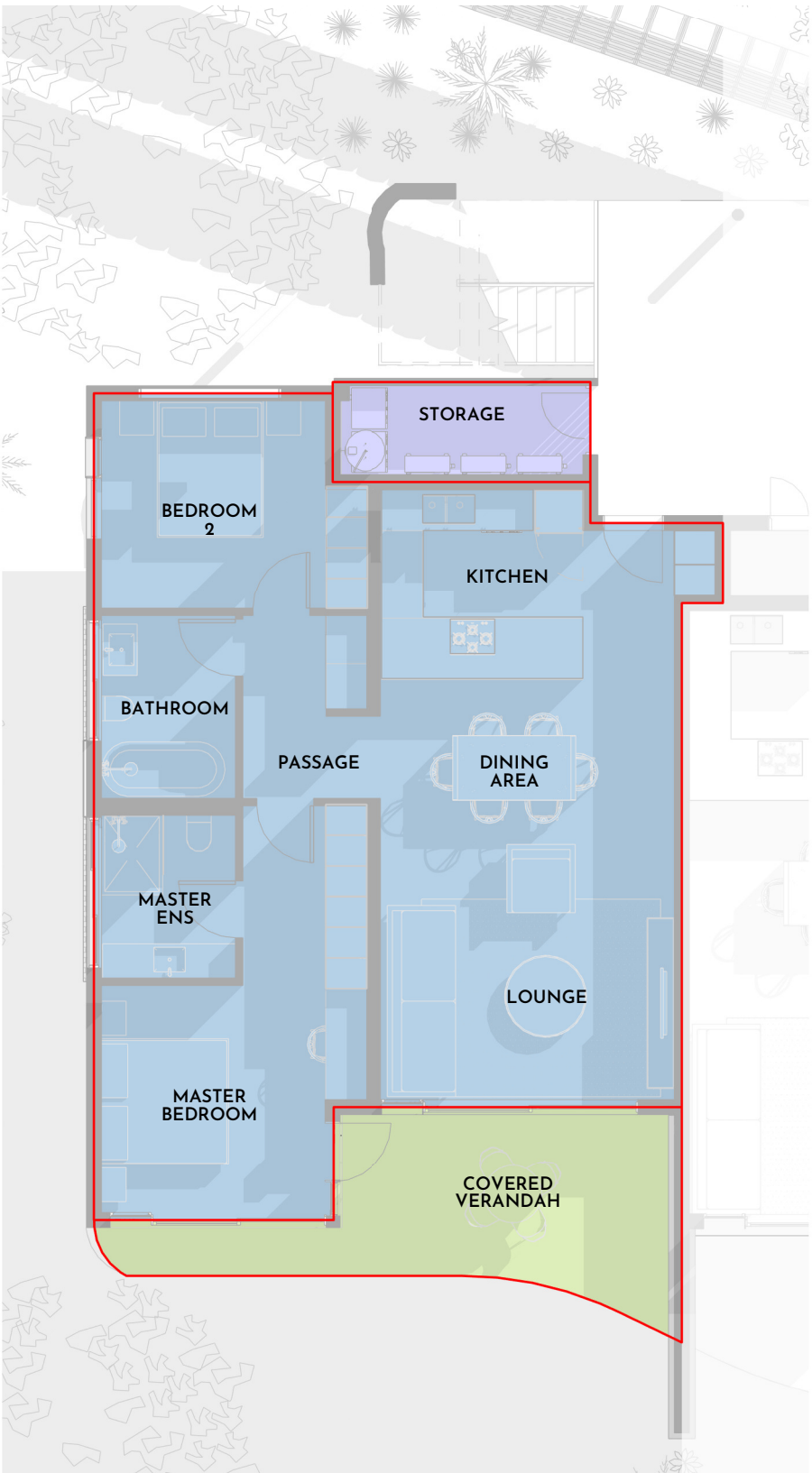
AREA - GROUND FLOOR - UNIT TYPE B- RIGHT SCALE 1 : 100
