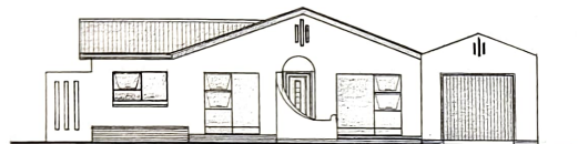
WEST ELEVATION
