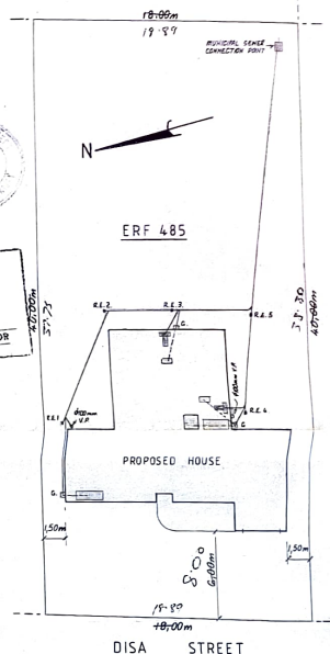
SITE & DRAINAGE PLAN
