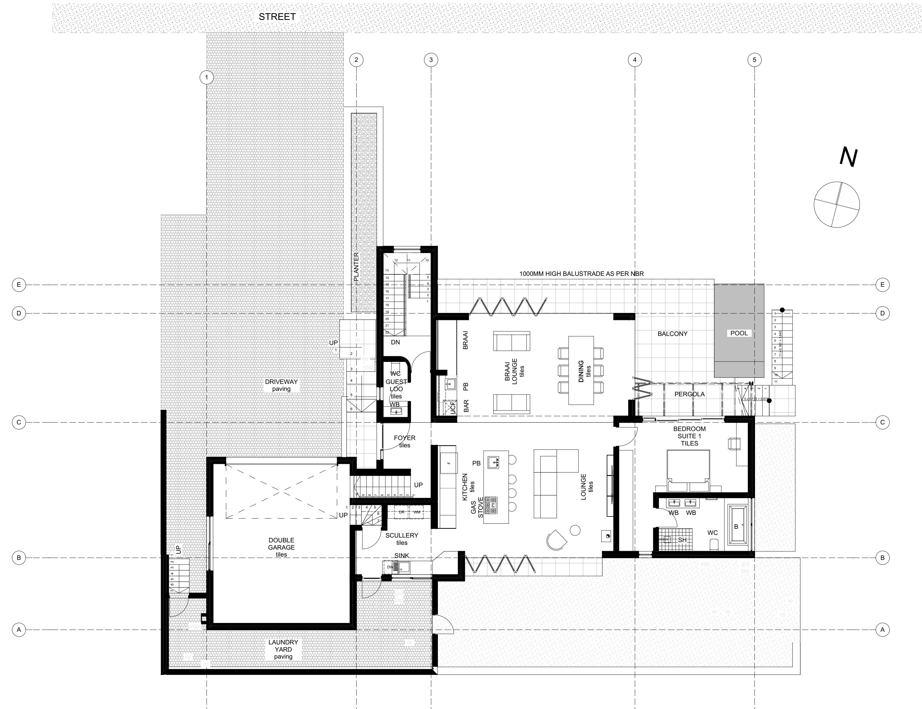
Ground Floor Scale 1:100
