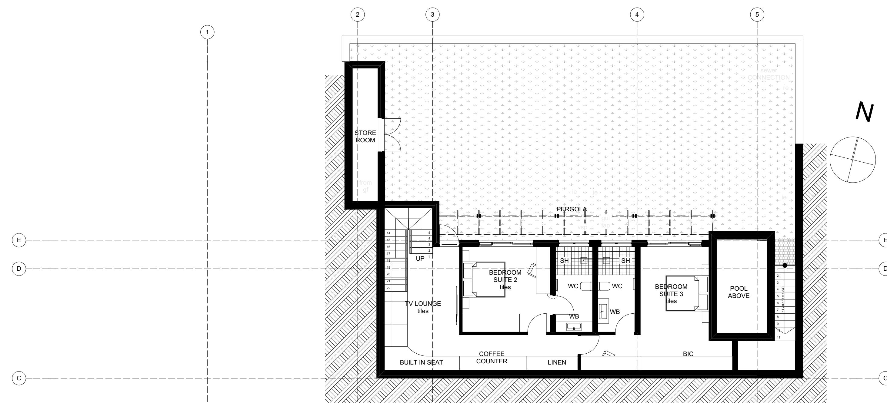
Lower Ground Floor Scale 1:100
