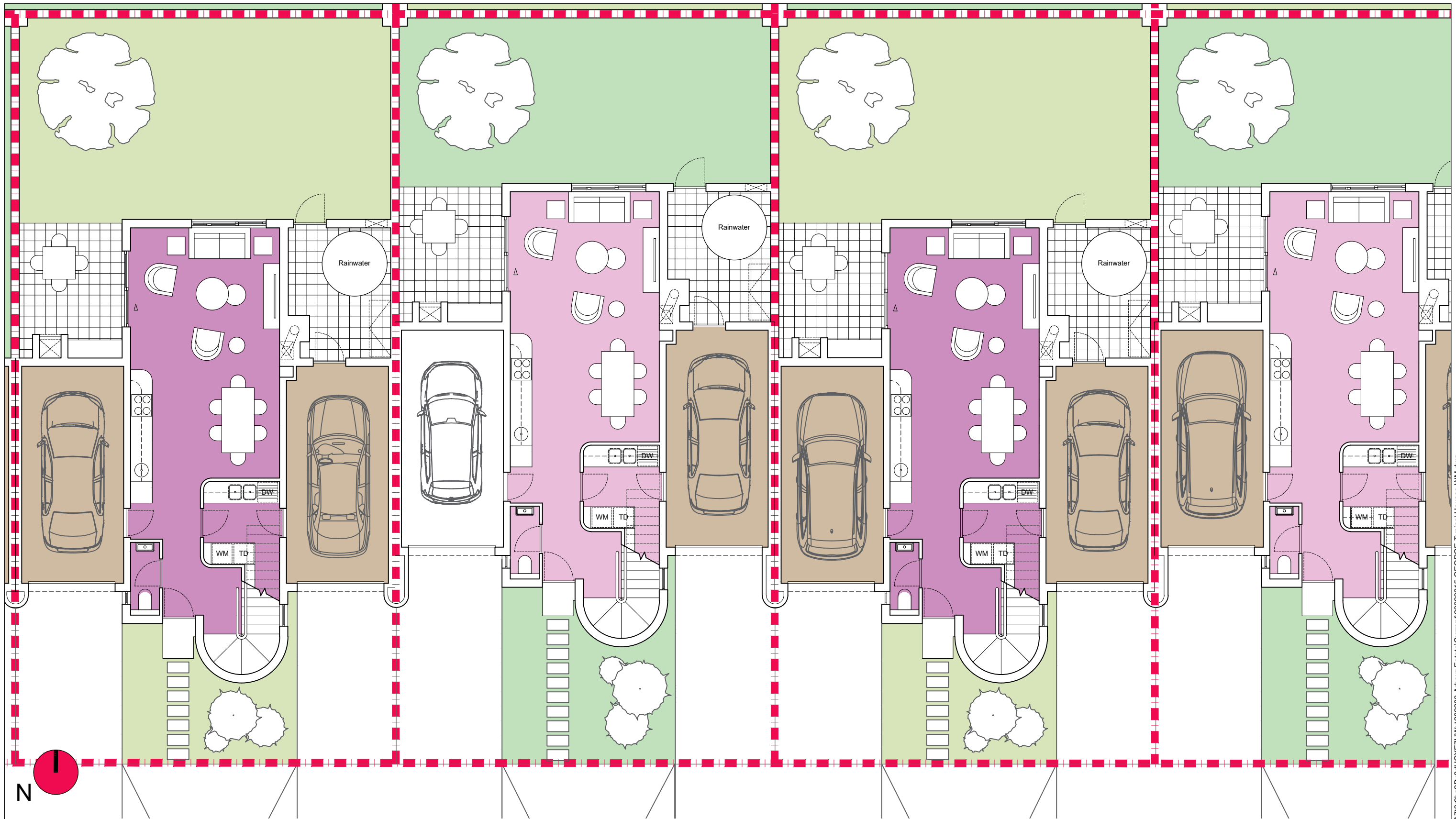
Ground Floor Plan (Scale 1:100 @ A3)
