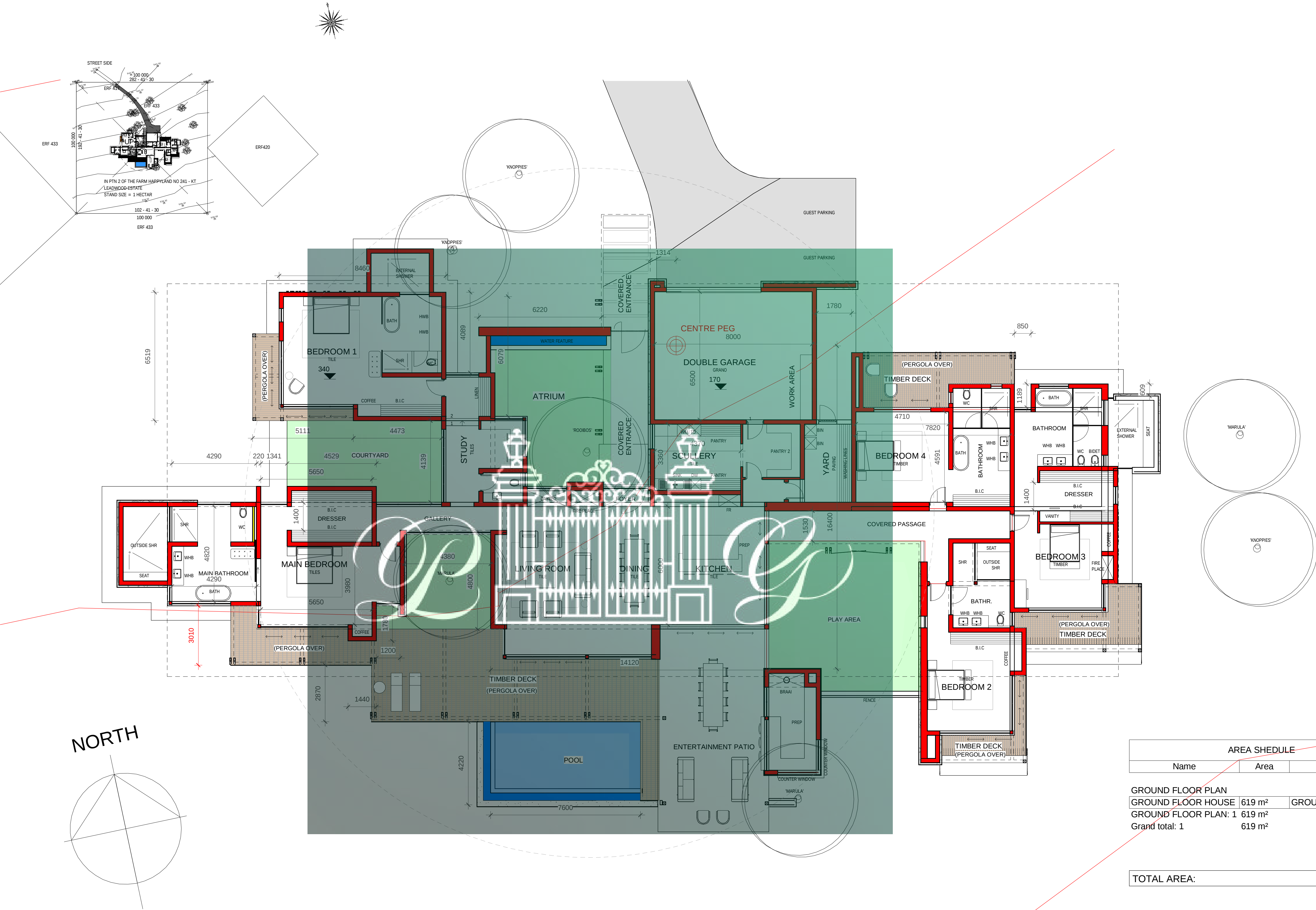
GROUND FLOOR PLAN 1 : 1500
