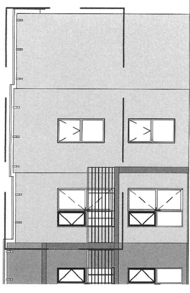
WEST ELEVATION SCALE - 1:100
