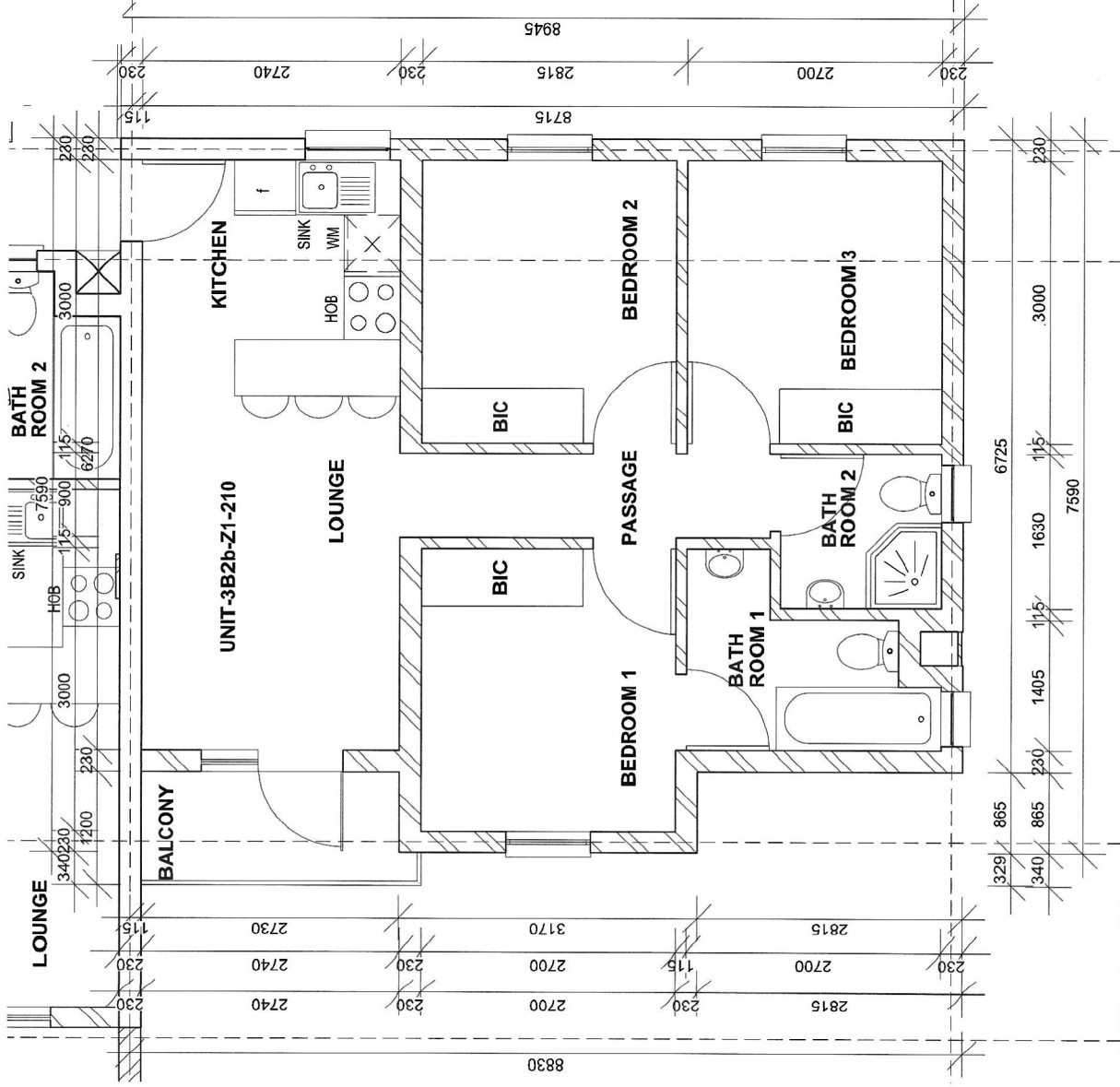
FIRST FLOOR PLAN SCALE - 1:50
