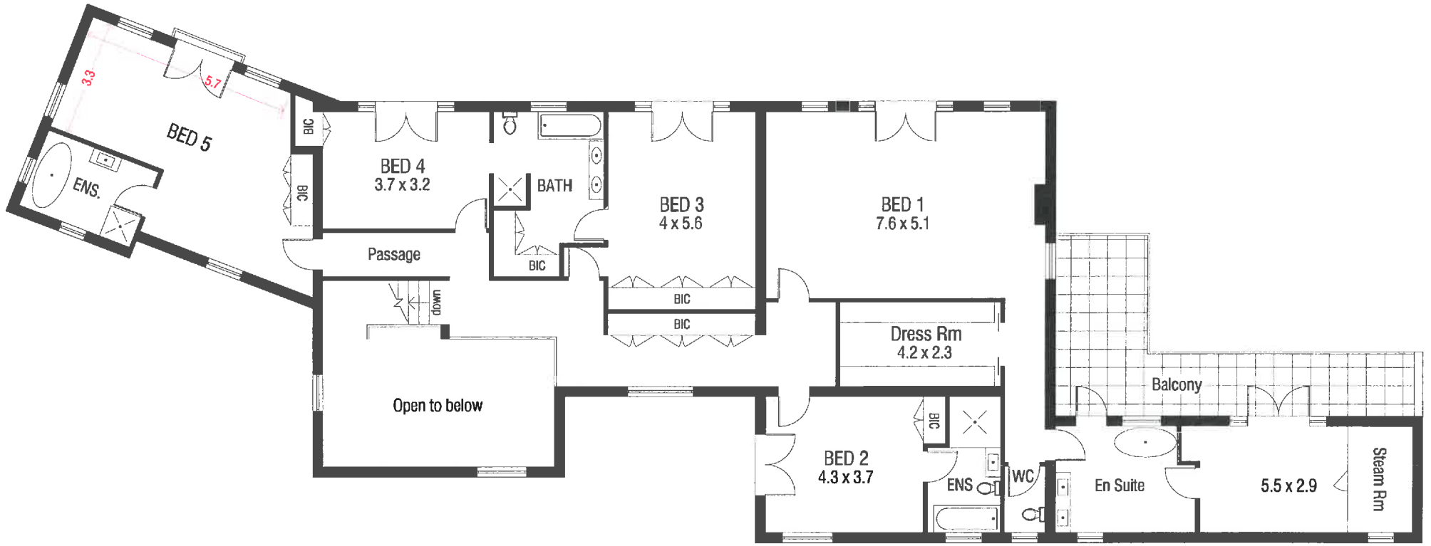
FIRST FLOOR
