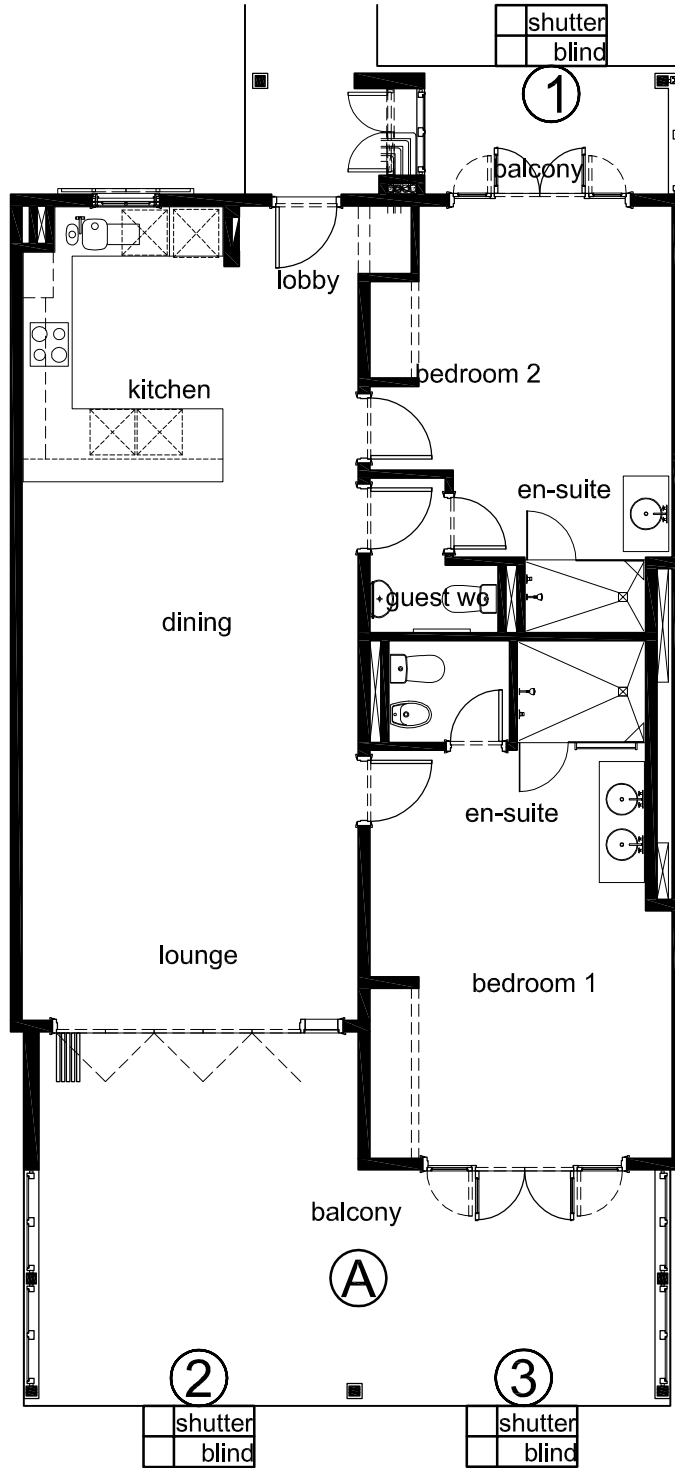
APARTMENT TYPE 11b
