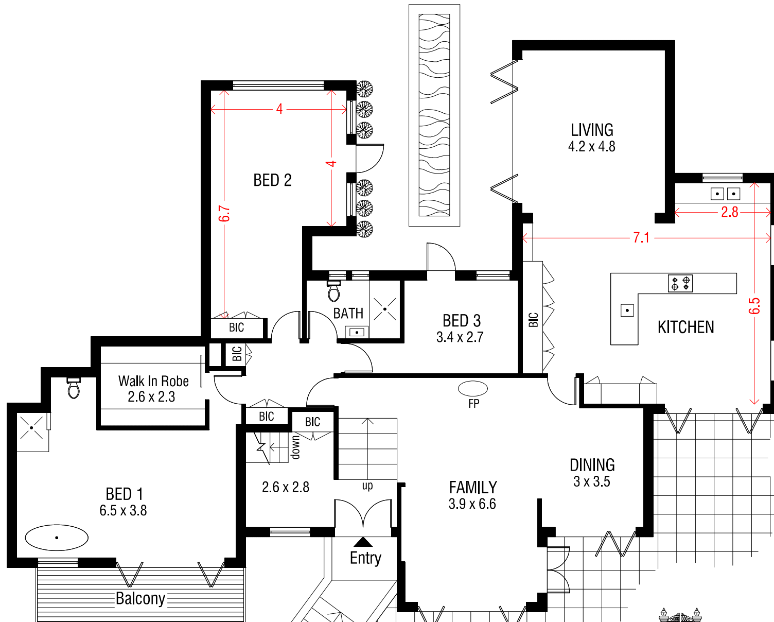
UPPER LEVEL
