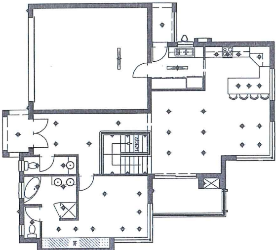
GROUND FLOOR PLAN 1:100 ELECTRICAL
