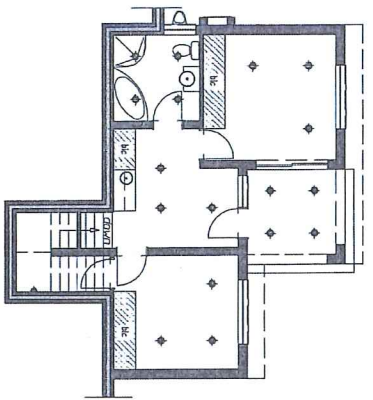
LOWER GROUND FLOOR PLAN 1:100 ELECTRICAL
