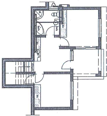
LOWER GROUND FLOOR PLAN 1:100 WATER SUPPLY
