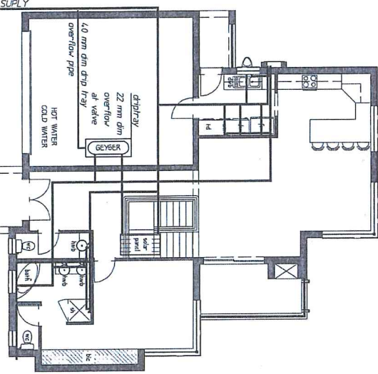
LOWER GROUND FLOOR PLAN 1:100 WATER SUPPLY
