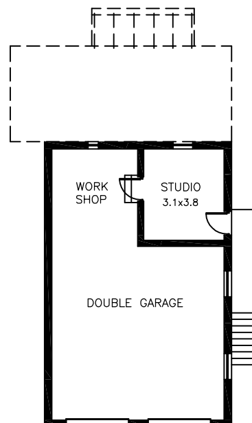
GARAGE PLAN SCALE 1: 200
