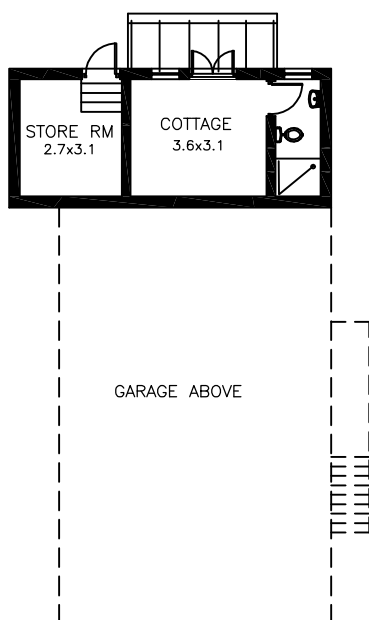
COTTAGE PLAN SCALE 1: 200
